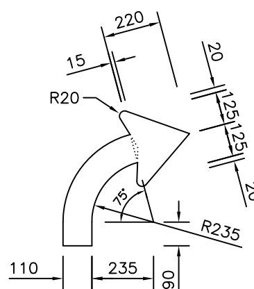
ARROW DETAILS
